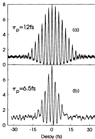
FIG. 4. Interferometric autocorrelation traces of nearly bandwidth-limited pulses (minimum-uncertainty wave packets) (a) incident on and (b) transmitted through the (HL) 11 sample.
