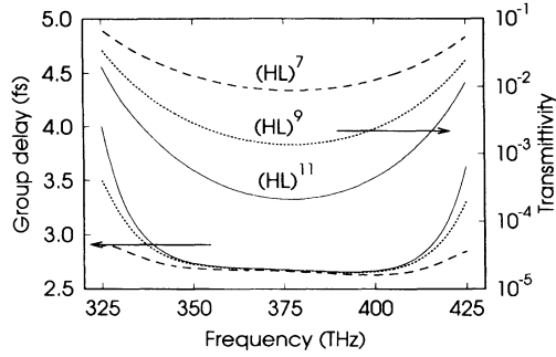
FIG. 1. Calculated group delay and intensity transmittivity versus frequency for quarter-wave multilayer dielectric mirrors consisting of quarter-wave layers of alternating low-index (L: fused silica) and high-index (H: titanium dioxide) transparent optical materials. The layer thicknesses were chosen to yield a photonic band gap centered at 375 THz ( \lambda = 0.8 \mu\text{m} ), coinciding with the carrier frequency of the wave packets used in our experiments.
