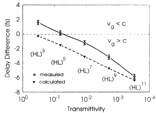
FIG. 3. Measured and calculated (for an angle of incidence of 20^\circ ) difference \Delta\tau between the tunneling time and the corresponding vacuum time for multilayer dielectric coatings of various thicknesses.
